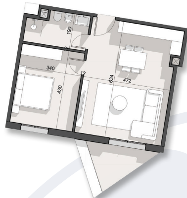
2D Floor Plan
